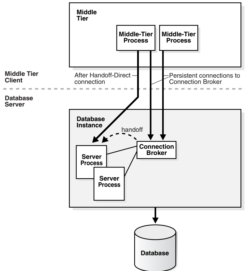
Figure 16–8 DRCP
