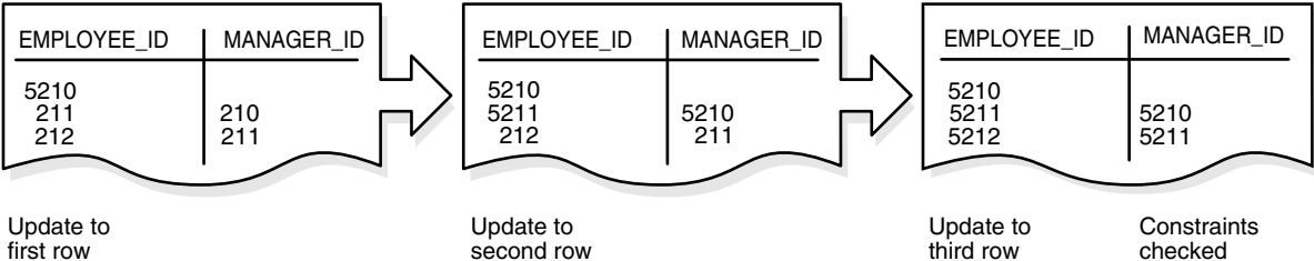
Figure 5-4 Constraint Checking
