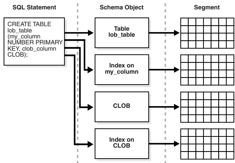
Figure 12–19 Multiple Segments
