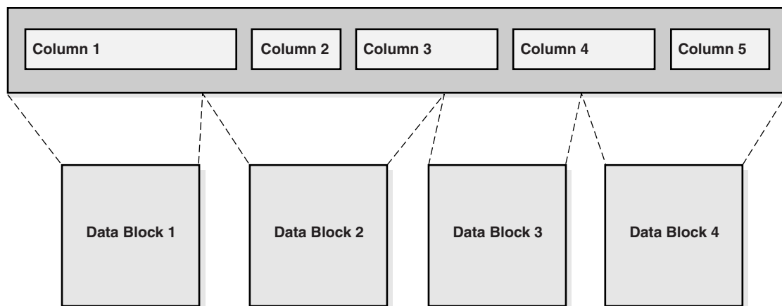
Figure 2–5 Compression Unit
