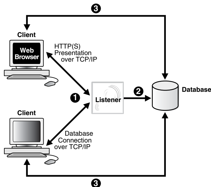
Figure 16-4 Listener Architecture
