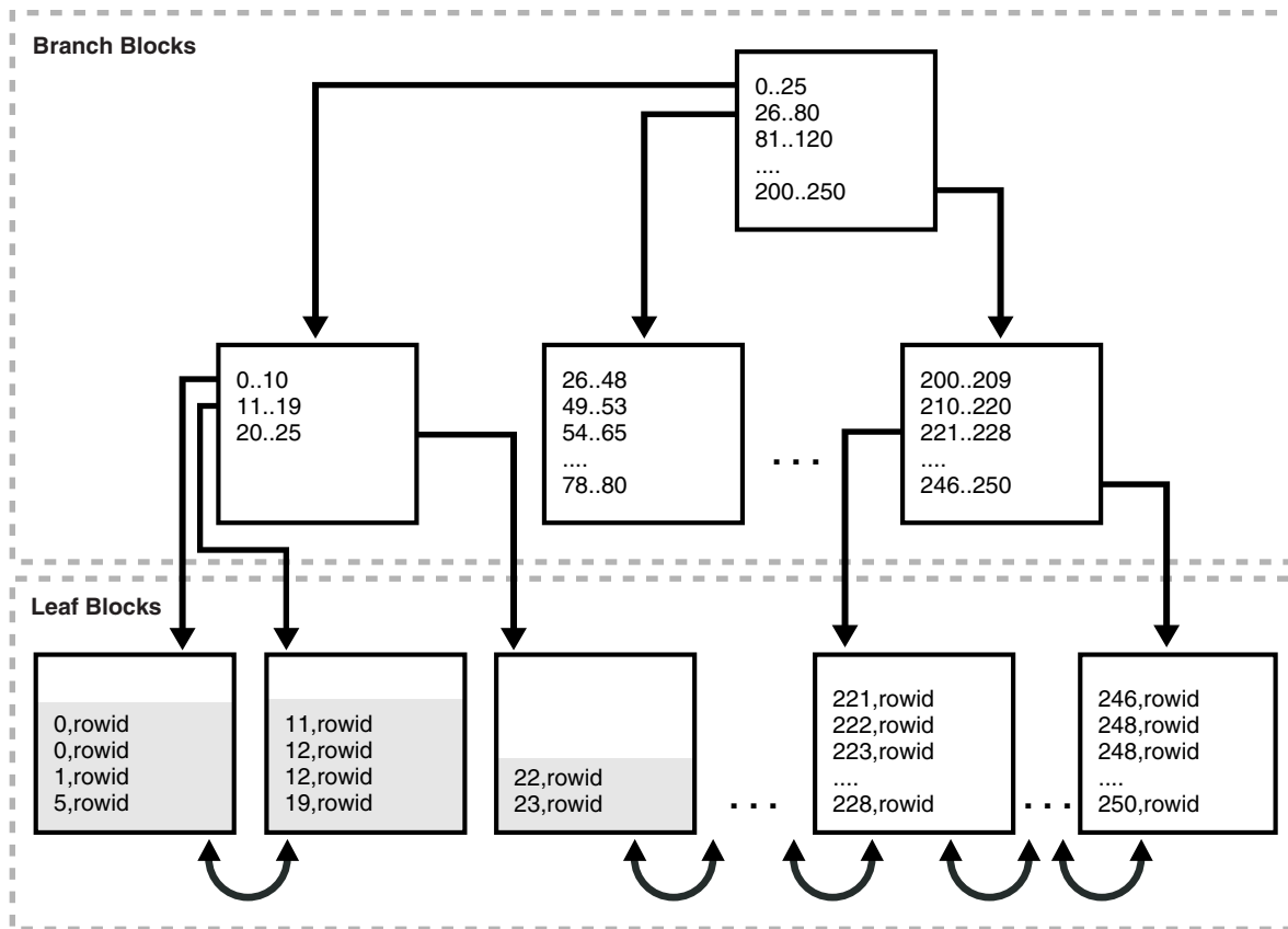
Figure 12-12 Index Before Coalescing
