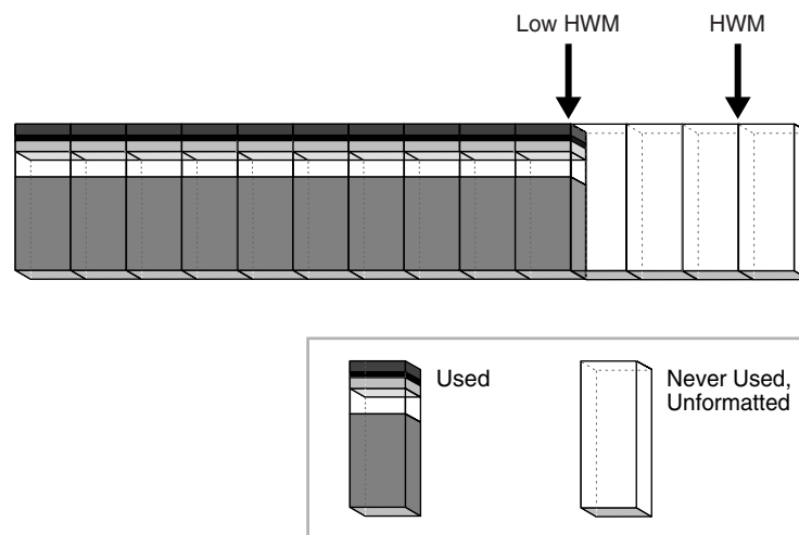
Figure 12–26 Advancing HWM and Low HWM
