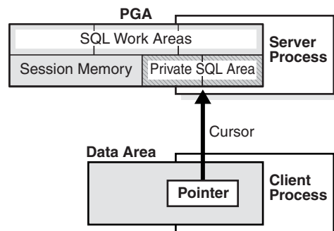
Figure 14–5 Cursor
