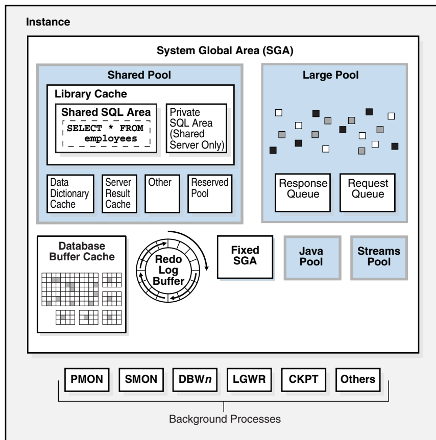
Figure 13–1 Database Instance
