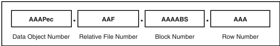
Figure 12-8 ROWID Format
